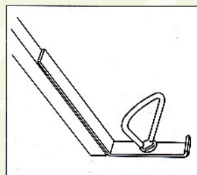
Stage Screw An alternative lower fixing for the extending brace. Material: Mild steel
