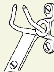
Brace Eye Designed to hold the extension brace to the rear surface of a scenery flat. Material: Malleable iron. Fixing: No. 8 Wood Screws
